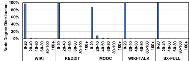
Figure 3. The distribution of nodes’ degree within the batch size of 900 in different datasets.
