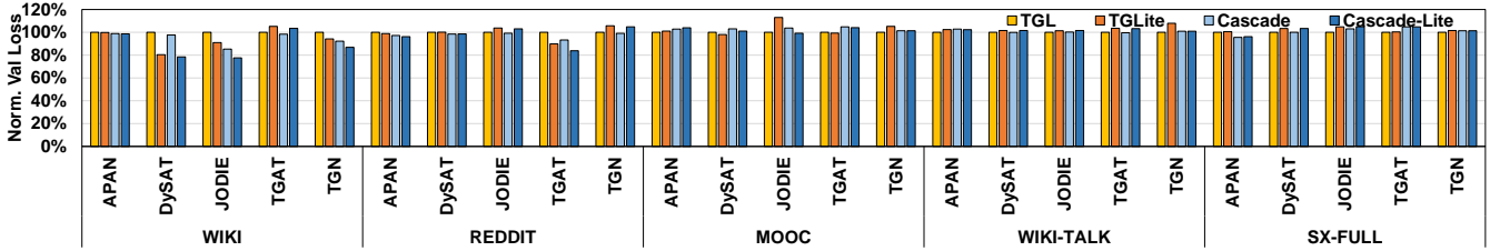
Figure 11. Validation losses (normalized to baseline) of TGNN models trained in Cascade and Cascade-Lite.
