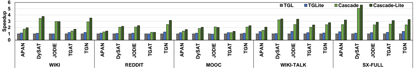
Figure 10. Training speed-ups introduced by Cascade and Cascade-Lite compared to baseline (TGL) and TGLite.
