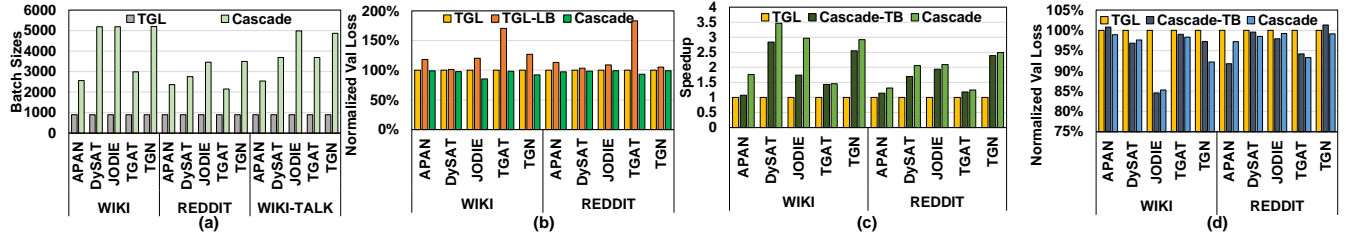
Figure 12. (a) Batch sizes of TGNNs in Cascade compared to the baseline. (b) Validation losses of TGNNs trained by Cascade and TGL-LB (baselines with larger batches)—results are normalized by the losses in the baseline. (c) Speedups of Cascade-TB and Cascade over baseline. (d) Validation losses of TGNNs trained in Cascade-TB and Cascade compared to baseline.
