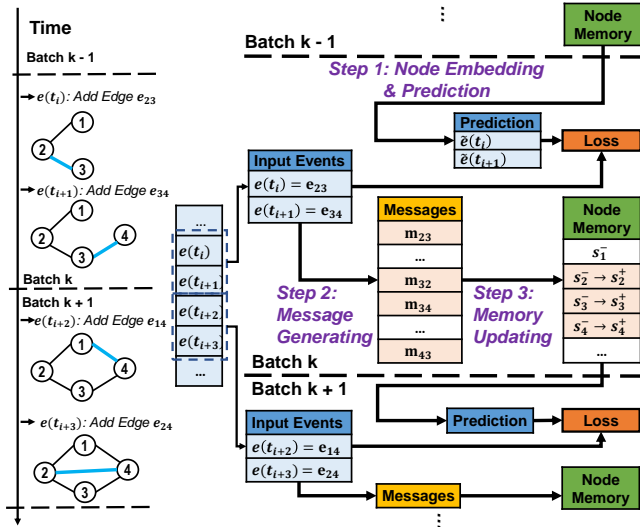
Figure 1. TGNN training steps: First start with node embedding and prediction, then message generating, and finally memory updating.
