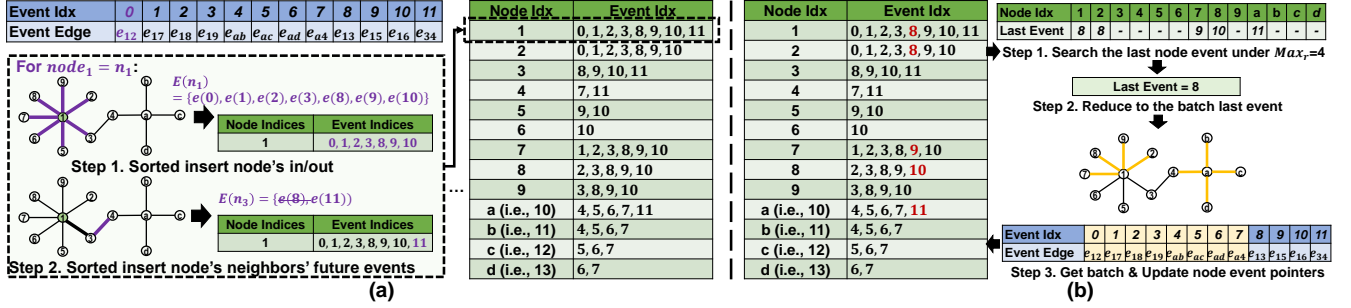
Figure 7. The workflow of TG-Diffuser: (a) Building dependency Table during preprocessing and (b) Looking up the last tolerable event during training.
