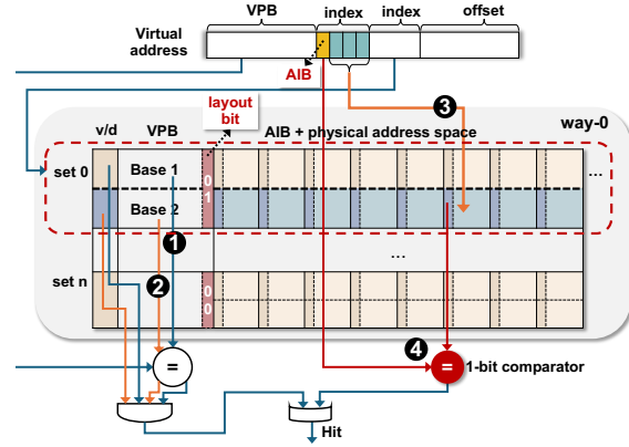
Fig. 9. TLB lookup process in STAR.
