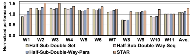
Fig. 18. Comparison of different TLB designs.
